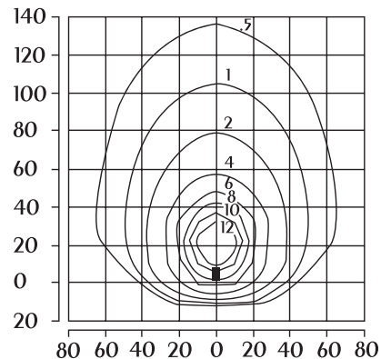
Isofootcandle plot of 1000W MH mounted at 30' w/ 60° tilt.
