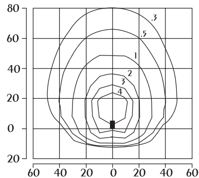
Isofootcandle plot of 400W MH mounted at 25' w/ 60° tilt.
